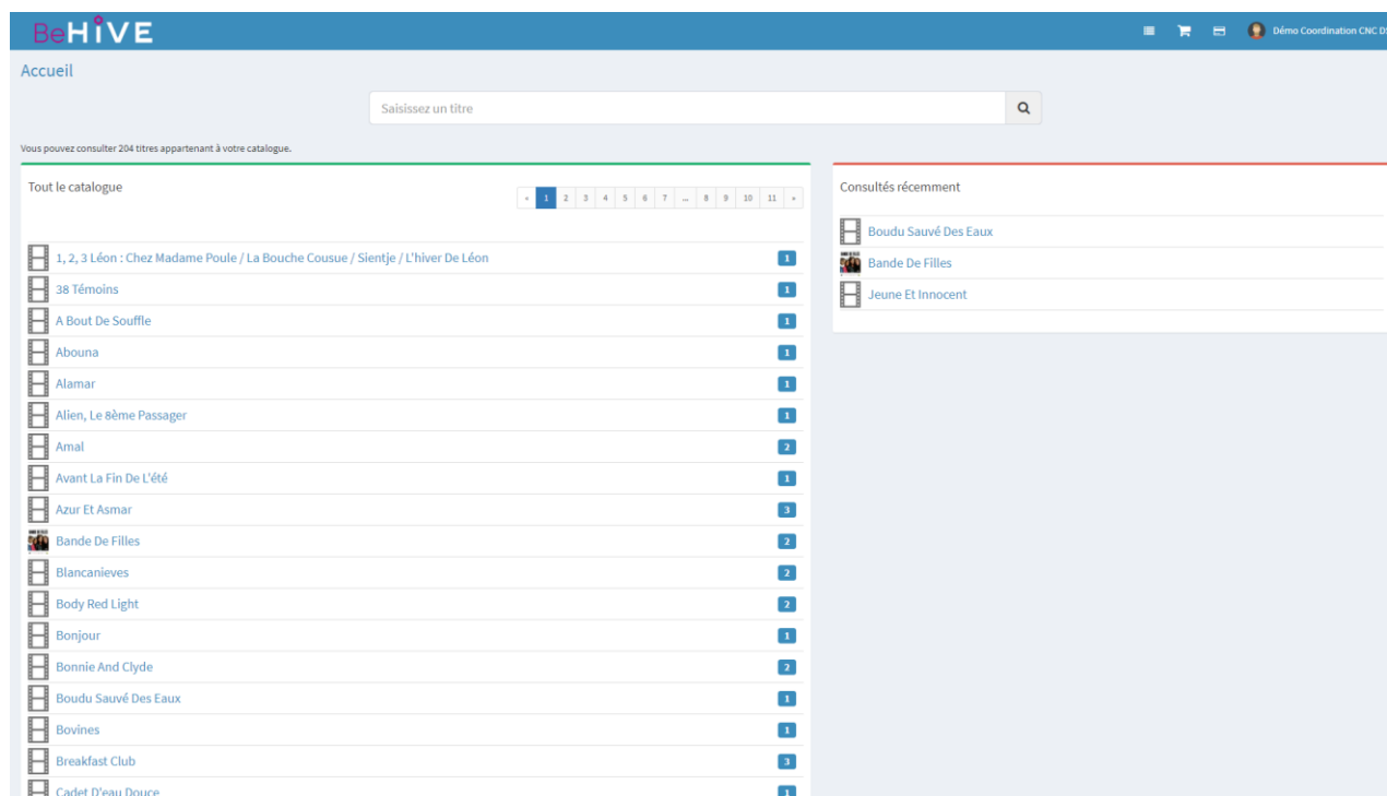
Figure 3 - BeHive catalogue
